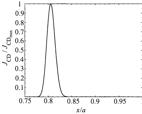
Figure 15.27 Normalized current profile as a function of normalized distance from the launcher. The profile peaks near the critical surface x/a = 0.81 .
