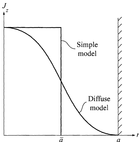
Figure 12.15 Simple model of a diffuse Z-pinch matching the current density on axis and the total current.
