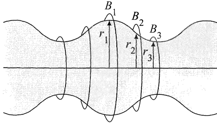
Figure 12.3 Schematic diagram of a Z-pinch interchange instability.
