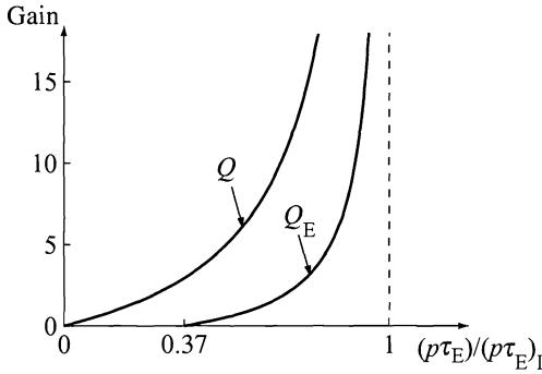
Figure 4.4 The physics gain factor Q and engineering gain factor Q_E as functions of (p\tau_E)/(p\tau_E)_1 .
