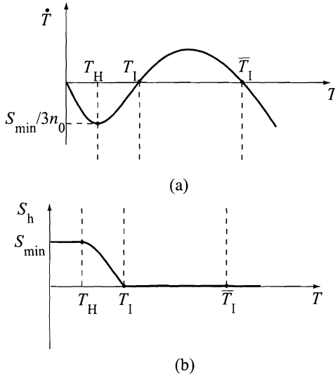
Figure 4.7 (a) \dot{T} vs. T showing the low ( T_I ) and high ( \bar{T}_I ) equilibrium points plus the negative minimum T = [S_a(T_H) - S_k(T_H)]/3n_0 = -S_{\min}/3n_0 . (b) Typical S_h(T) vs. T profile that vanishes at S_h(T_I) = 0 and whose value at T = T_H satisfies S_h(T_H) \geq S_{\min} .
