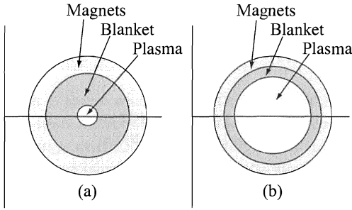
Figure 5.9 Low efficiency of the blanket because of: (a) too small a plasma, and (b) too large a plasma leading to low power density.
