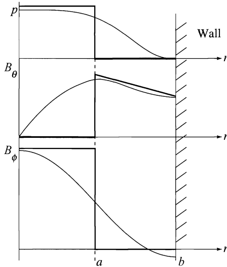
Figure 13.13 Surface current model approximating the RFP configuration.
