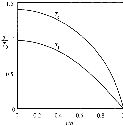
Figure 14.6 T_e and T_i vs. r/a for \alpha = 10 , \chi_i/\chi_e = 10 .
