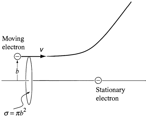
Figure 7.3 Strong Coulomb interactions occurring when m_e v^2/2 \approx e^2/4\pi \epsilon_0 b .
