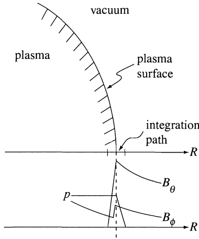
Figure 13.10 Integration across the plasma–vacuum interface.
