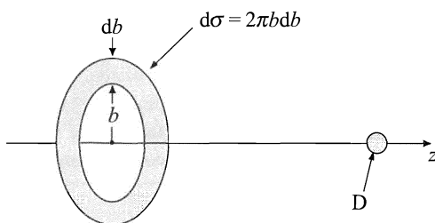
Figure 3.5 Illustration of the differential cross section d\sigma = 2\pi b db .
