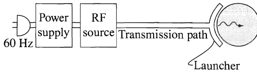
Figure 15.7 Schematic diagram of an RF heating or current-drive system.
