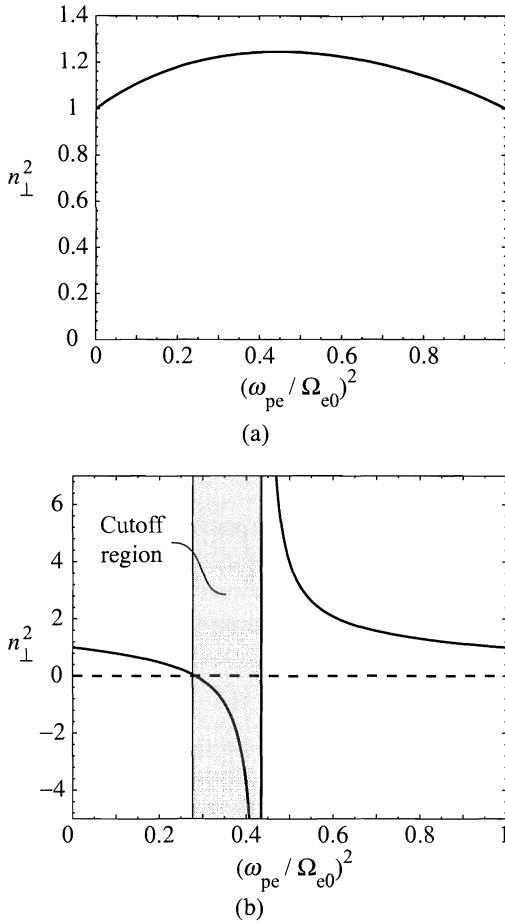
Figure 15.19 (a) Dispersion relation for the fundamental ECH X mode assuming a high-field, inside launch for the case \varepsilon = 1/3 . There is good accessibility from the launch site to the center of the plasma. (b) The same dispersion relation for the low-field launch. Observe the cutoff and wave resonance at low \omega_{pe}^2/\Omega_{e0}^2 .
