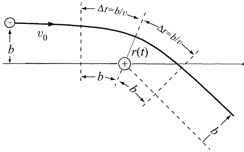
Figure 3.12 Geometry of a Coulomb collision.
