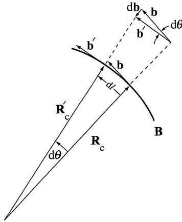
Figure 8.8 Geometry showing the relation between \mathbf{b} \cdot \nabla \mathbf{b} and \mathbf{R}_c . Here, \mathbf{b} = \mathbf{b}(\mathbf{r}_{\perp}, l) and \mathbf{b}' = \mathbf{b}(\mathbf{r}_{\perp}, l + dl) . Similarly for \mathbf{R}_c and \mathbf{R}'_c .
