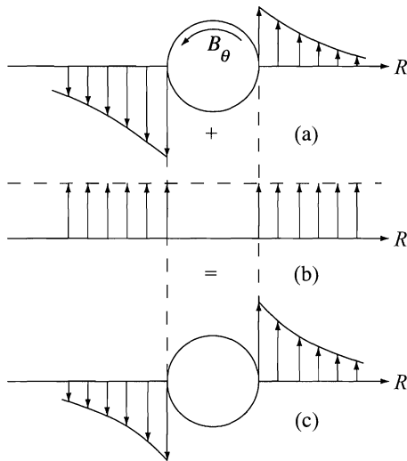
Figure 11.23 Physical picture of the vertical field restoring force: (a) original plasma showing the B_\theta imbalance on the inside and outside; (b) add a pure vertical field in the direction shown; (c) the combination balances B_\theta on the inside and outside providing toroidal force balance.
