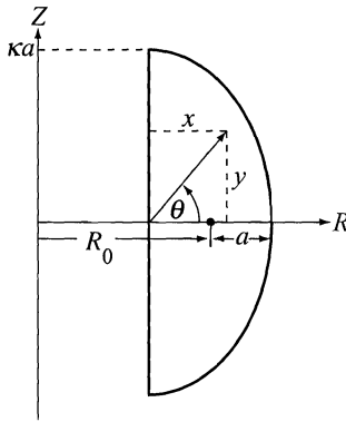
Figure 13.37 Non-circular half-ellipse model for the ST plasma.
