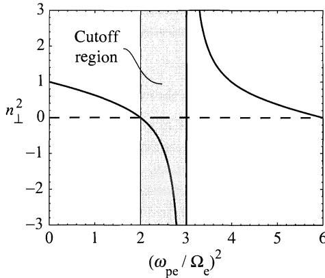
Figure 15.20 Dispersion relation for the second harmonic ECH X mode assuming a low-field, outside launch and \varepsilon = 1/3 . Observe that there is good accessibility for \omega_{pe}^2/\Omega_e^2 < 2 .
