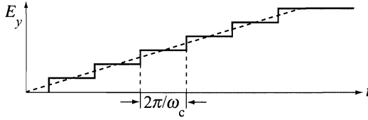
Figure 8.9 Dashed curve: linearly rising electric field that levels off after a period of time. Solid curve: step function model of the electric field evolution.
