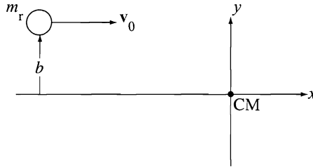
Figure 9.3 Center of mass (CM) geometry showing how to calculate E_0 and L_0 in terms of b and \mathbf{v}_0 .
