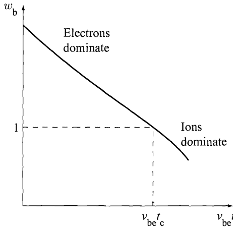
Figure 9.11 Normalized beam velocity w_b = v_b/v_c as a function of time.
