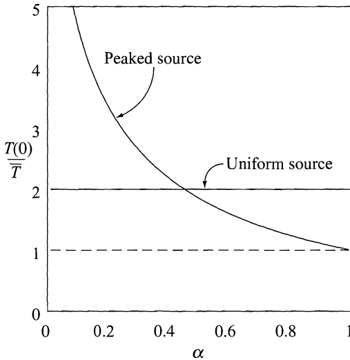
Figure 14.8 Peaking factor vs. normalized localization radius.
