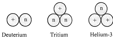
Figure 2.1 Nuclear structure of the basic fusion fuels.
