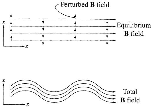
Figure 12.10 The shear Alfvén wave showing field-line bending.
