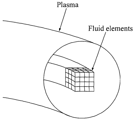
Figure 10.1 Subdividing a plasma into small fluid elements.
