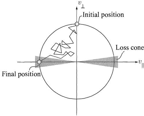
Figure 9.8 A particle starting from its initial position in velocity space is lost instantaneously once it diffuses into the loss cone as a result of many small-angle collisions.
