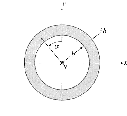
Figure 9.7 Transverse plane showing the angle \alpha .
