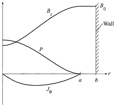
Figure 11.13 Typical \theta -pinch profiles.
