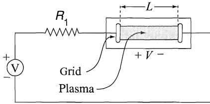
Figure 7.1 Idealized circuit diagram to examine Debye shielding.
