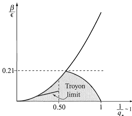
Figure 13.28 The Troyon limit superimposed on the surface current stability diagram.
