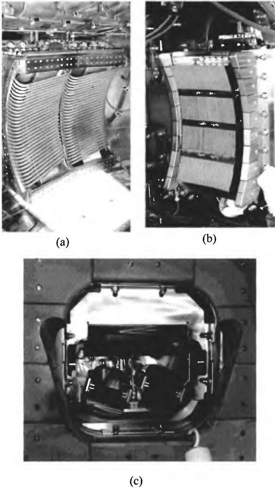
Figure 15.10 Launching structures for: (a) an ICH antenna (courtesy of E. Marmor), (b) an LHCD waveguide array (courtesy of E. Marmor), (c) an ECH mirroring system (Lohr, J. et al. , (2005). Fusion Science and Technology , 48 , 1226).
