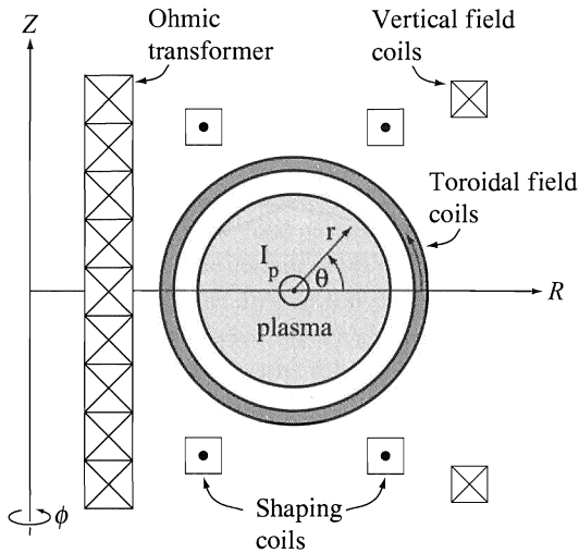
Figure 13.22 Schematic diagram of a tokamak.
