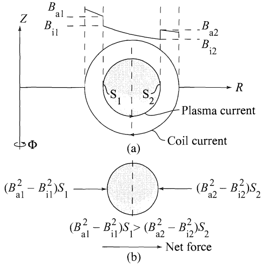
Figure 11.19 Qualitative picture of the 1/R force: (a) surface current model showing the 1/R dependence of B_\phi along the midplane Z=0 ; (b) toroidal force balance showing a net outward force along R .
