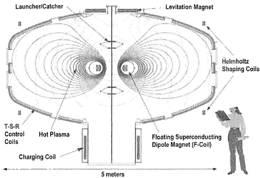
Figure 13.1 Conceptual drawing of the LDX experiment (courtesy of D. Garnier).
