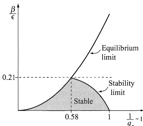
Figure 13.26 Overall stability diagram for the surface current model of a circular tokamak showing the equilibrium limit and the numerically computed stability limit (D'Ippolito et al. (1976). Plasma Physics and Controlled Nuclear Fusion Research , 1 , 523).
