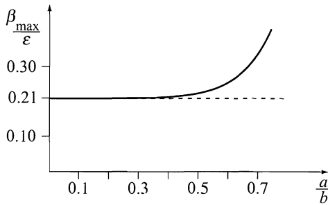
Figure 13.35 Curve of \beta_{\max}/\epsilon vs. a/b showing how the \beta limit increases as the wall is moved closer to the plasma.
