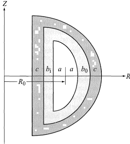
Figure 13.40 Geometry of a fusion neutron source.
