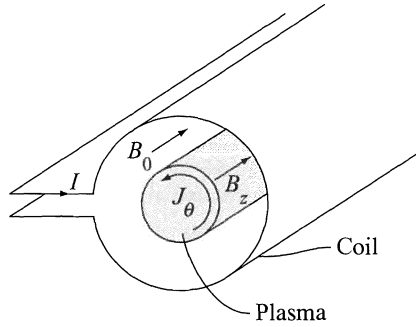
Figure 11.12 Schematic diagram of a \theta -pinch.
