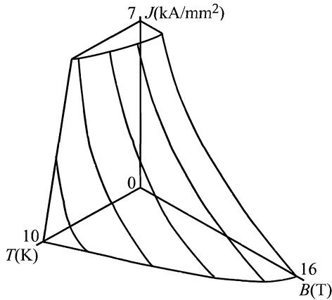
Figure 5.3 The 3-D T, J, B dome for niobium–tin under which a superconducting magnet must operate to be in its superconducting state (Wilson, M. N. (1983). Superconducting Magnets Oxford: Clarendon Press).
