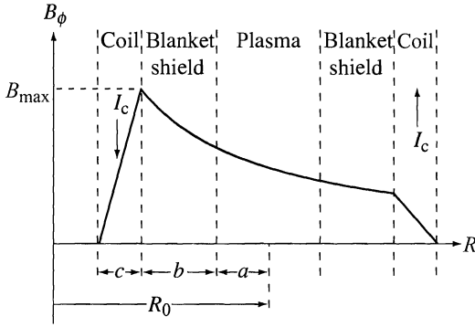
Figure 13.39 Geometry of a tokamak reactor showing the location of B_{\max} . Note that B_{\phi} vanishes outside of the toroidal field coil.
