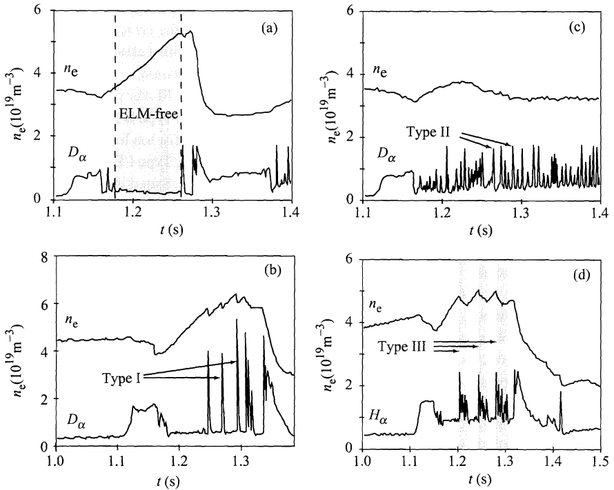
Figure 14.20 Experimentally measured electron density and D_\alpha or H_\alpha emission time histories showing: (a) ELM-free operation and (b) type I, (c) type II, and (d) type III ELMs (ASDEX Team. (1989). Nuclear Fusion , 29 , 1959).
