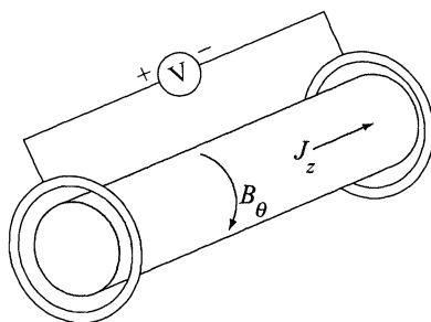
Figure 11.14 Schematic diagram of a Z-pinch.
