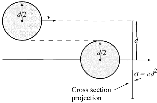
Figure 3.6 Hard-sphere collision cross section \sigma = \pi d^2 .
