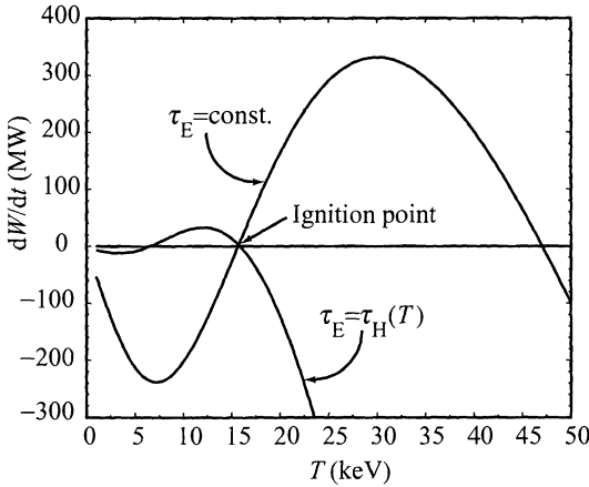
Figure 14.25 dW/dt vs T for \tau_E = \tau_H(T) and \tau_E = \text{const.} = 1.2 assuming P_h = 0 .
