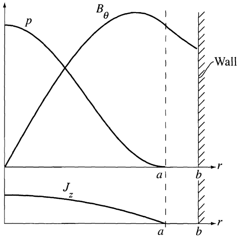
Figure 11.15 Typical Z-pinch profiles.
