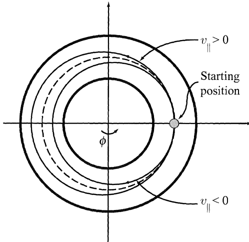
Figure 14.16 Top view of the tokamak showing the toroidal projection of two passing particle orbits, one with v_{\parallel} > 0 , the other with v_{\parallel} < 0 . Note that the radius of the v_{\parallel} < 0 orbit is the smaller, implying that if \partial n / \partial r < 0 there will be a downward magnetization current at the point of tangency.
