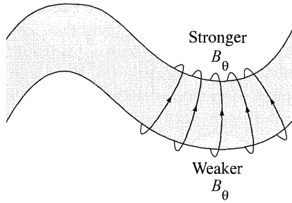
Figure 12.4 Schematic diagram of a twisting Z-pinch instability.
