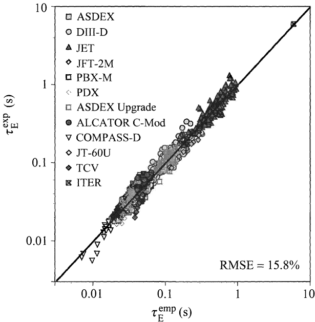
Figure 14.22 Comparison of experimental and empirical \tau_E for the H-mode scaling relation (ITER Physics Experts Groups on Confinement Modelling and Database (1998). Nuclear Fusion , 39 , 2175).
