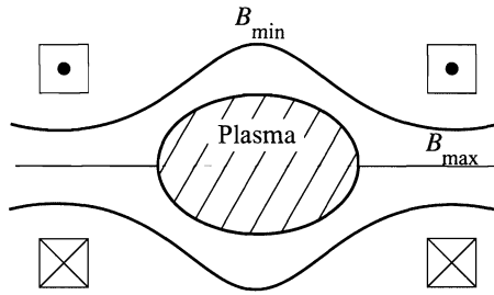
Figure 8.16 Geometry of the simple mirror machine.
